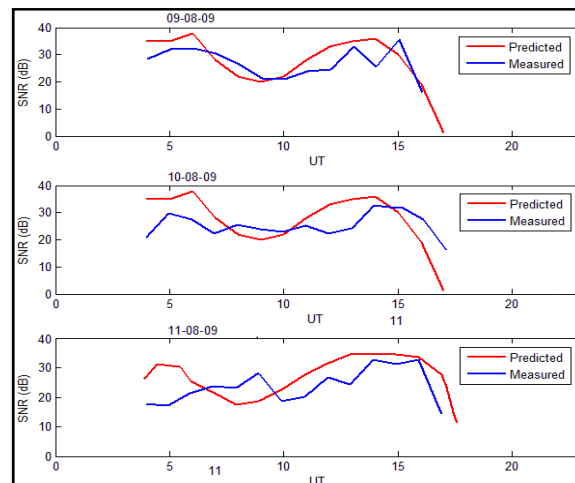
Figure 8.Comparison of predicted and measured SNR for 9, 10, 11 September 2009 on 14.10 MHz
