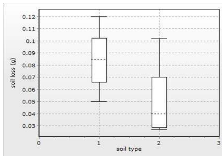
Figure 2: Comparison of mean soil losses between Lab Sand (1) and Woburn soil (2) at rainfall intensity of 120 mm/hr
