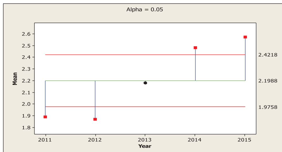
Figure A5. One-way normal ANOM for annual price (2011–2015).
