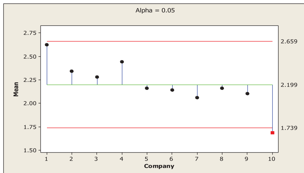
Figure A4. One-way normal ANOM for price by company.
