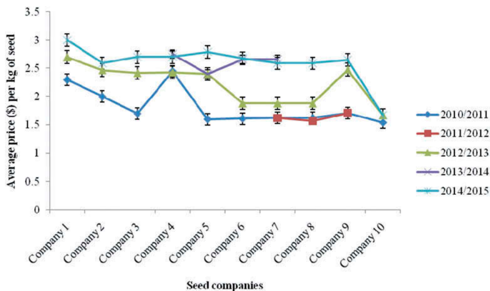
Figure 4. Annual mean prices for hybrid maize seed.
