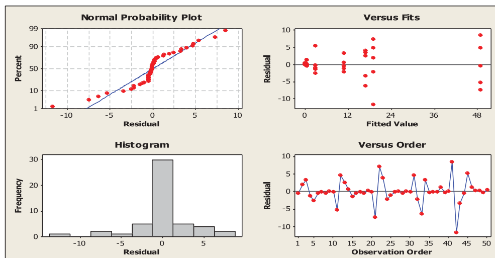
Figure A2. Residual plots for % market share.
